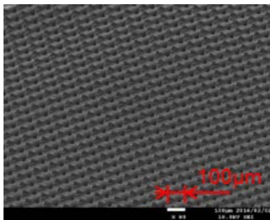
(Foil with micro hole, 220holes/mm 2 )
